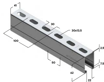
41x62
