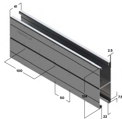
41x124
